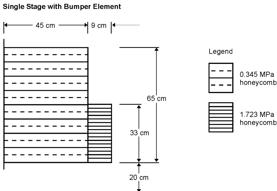
Figure 3 Deformable Barrier Face Profile and Dimensions
